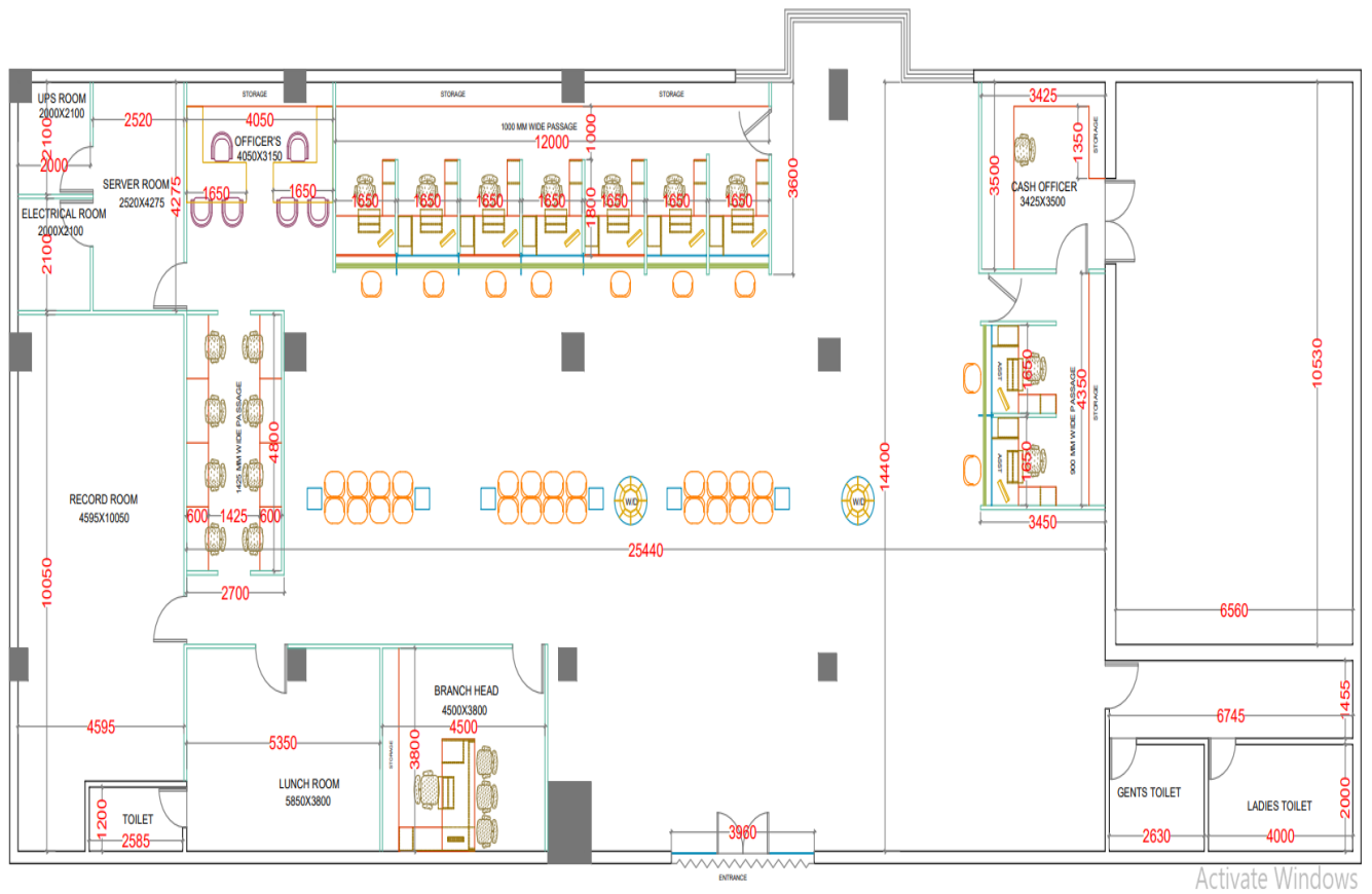
DRAWING: - TREASURY BRANCH (2016) UNDER RBO HIMAYATH NAGAR, AO SE-CUNDERABAD
